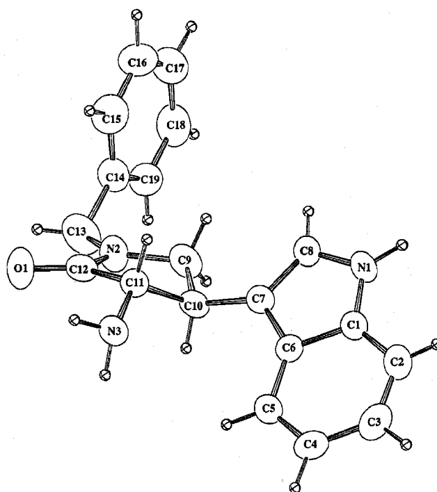
Figure 1. Molecular structure of compound 18b as determined by X-ray diffraction; the numbering does not correspond to the systematic name
